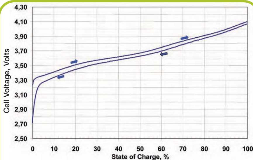
Figure 2: Typical Li-ion voltage profile (LiNixCoyAlzO 2 /graphite system). Charge/discharge curves at low rate
