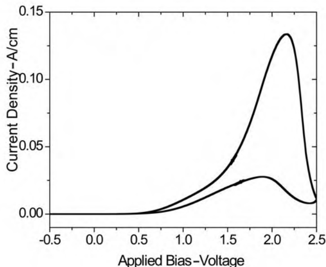
The current density versus voltage curve for organic switches using NDR
