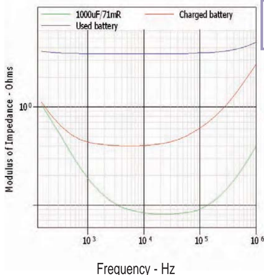
Figure 8: Battery impedance; two Ni-MH AA cells
