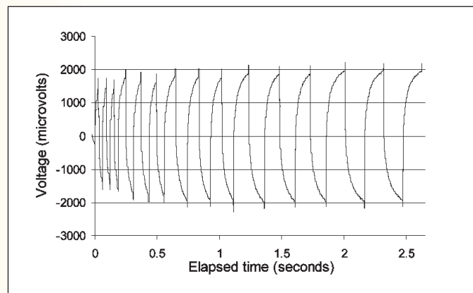
Figure 4d: Voltage response with the underlying micro-discharge 'drift' removed
