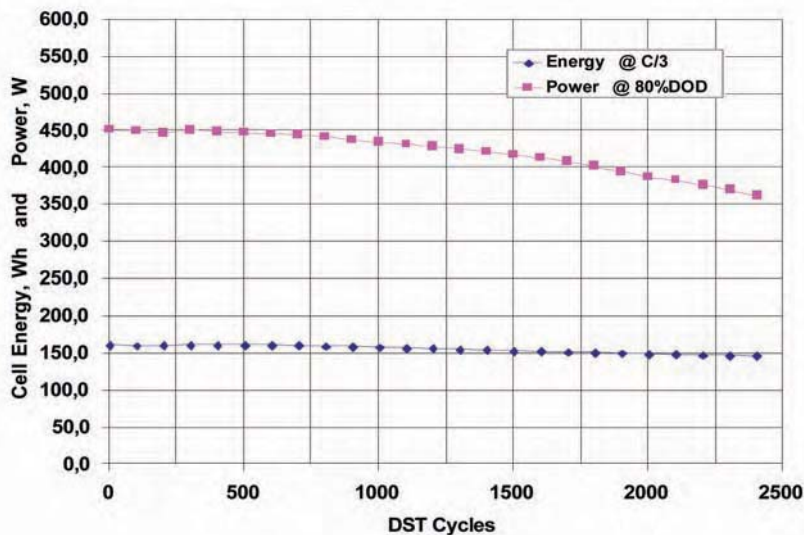
Figure 5: Energy and power evolution of Saft "VL45E" cells during cycling at 80% DOD DST cycle. Every 50 cycles, energy measured at 100% DOD – C/3, power measured at 80% DOD, 300A – 5mm pulse
