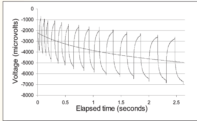
Figure 4c: Pulse pattern design for a predictable underlying shift, with custom-modelled trend line
