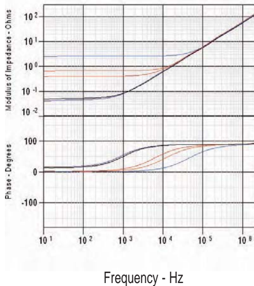
Figure 12a and 12b: Impedance response of inductors
