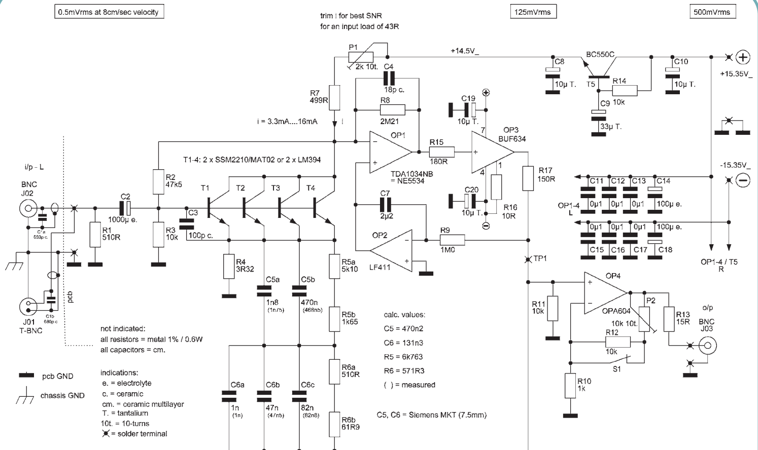
Figure 4: Solid-state MC-RIAA pre-amp
