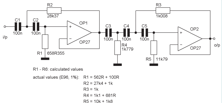
Figure 1: S-filter with hp cut-off frequency of 355Hz
