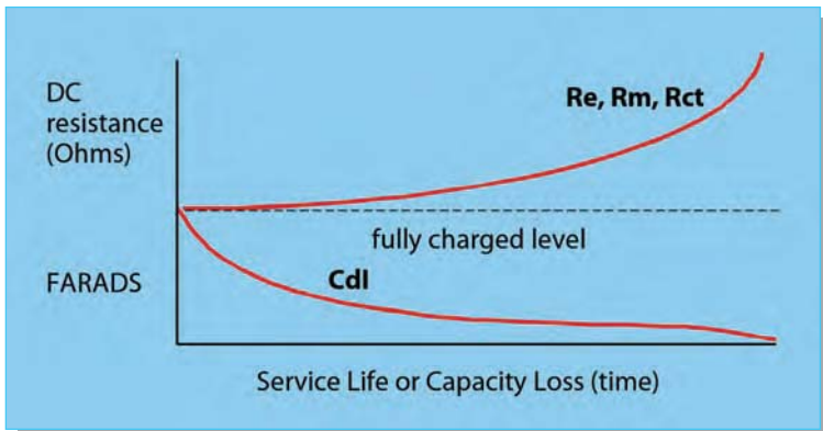
Figure 3: Randles parameter progression over the cell lifetime or discharge
