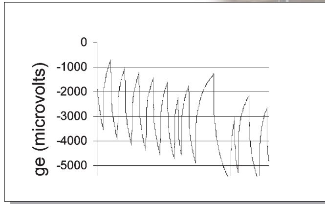
Figure 4a: A typical voltage 'micro discharge' characteristic for a current 'shorting only' random pulse pattern
