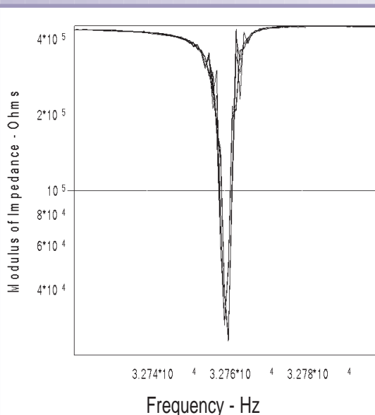
Figure 3: Response of a 32768Hz crystal
