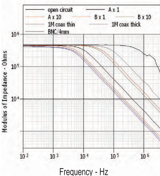
Figure 9: Scope probe impedance
