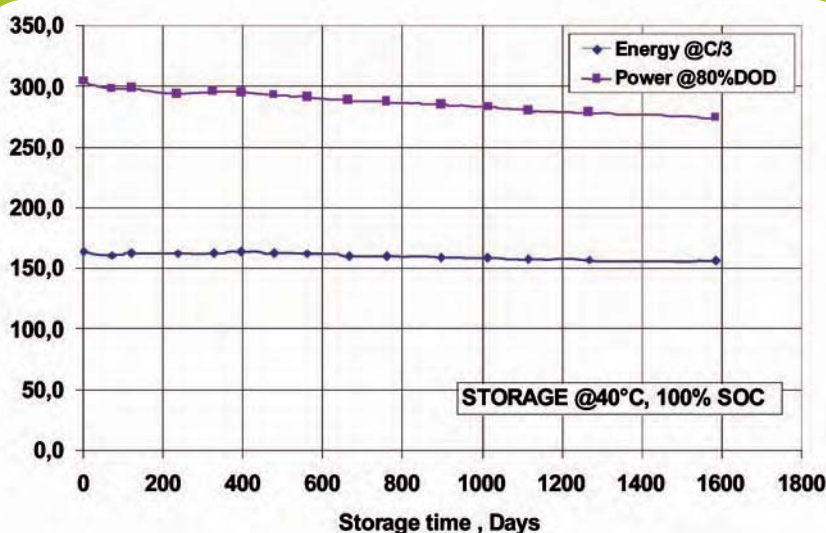
Figure 3: Example of energy and power retention of large 45Ah Li-ion cells VLE45 during extended high temperature storage at full state-of-charge
