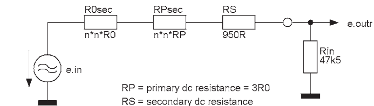
Figure 3b: Transformer circuit's equivalent
