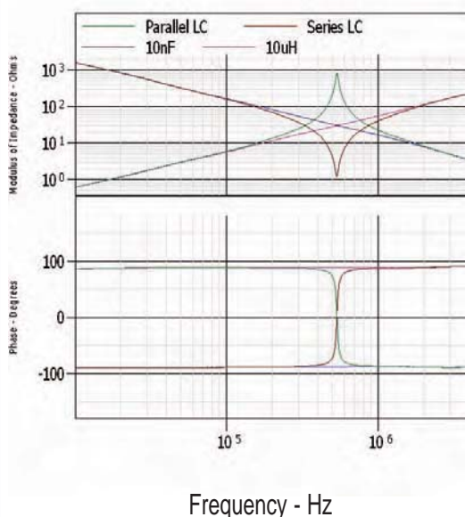
Figure 13a and 13b: Response of resonant circuits
