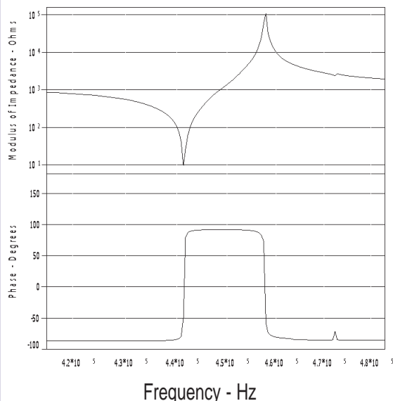
Figure 2: Complex response of a 455KHz resonator
