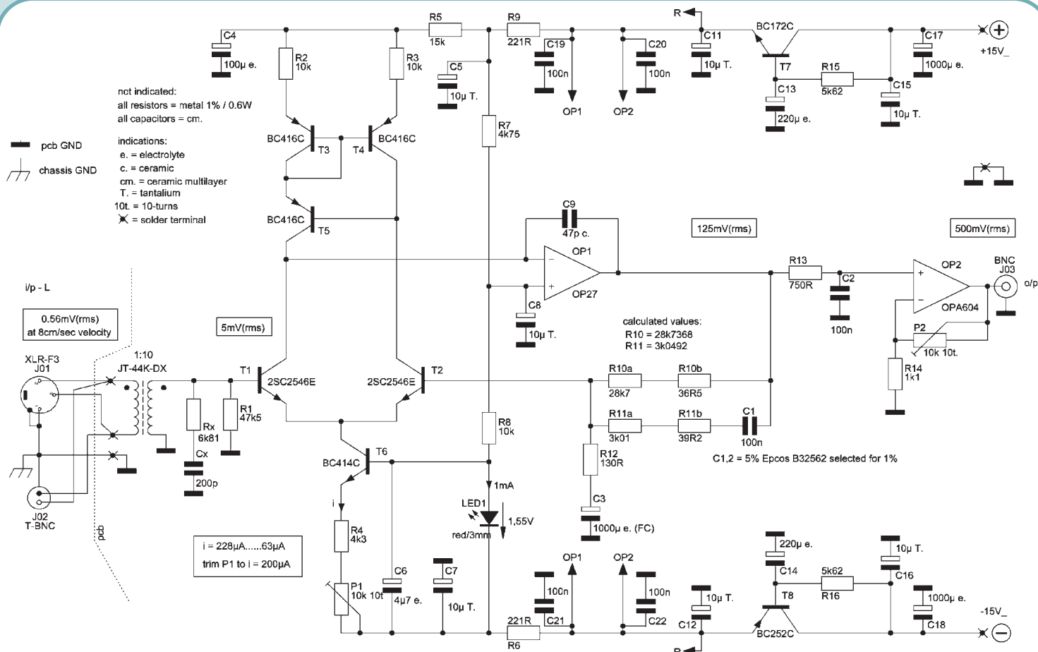
Figure 2: MC-RIAA pre-amp formed by a step-up transformer plus BUVO-MM-RIAA pre-amp
