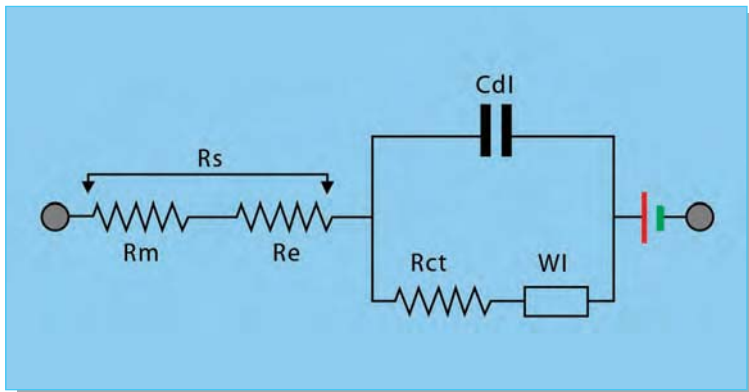
Figure 2: The Randles equivalent circuit for an electrochemical cell
