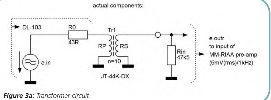
Figure 3a: Transformer circuit
