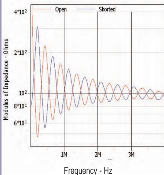
Figure 7: Response of a USB cable impedance
