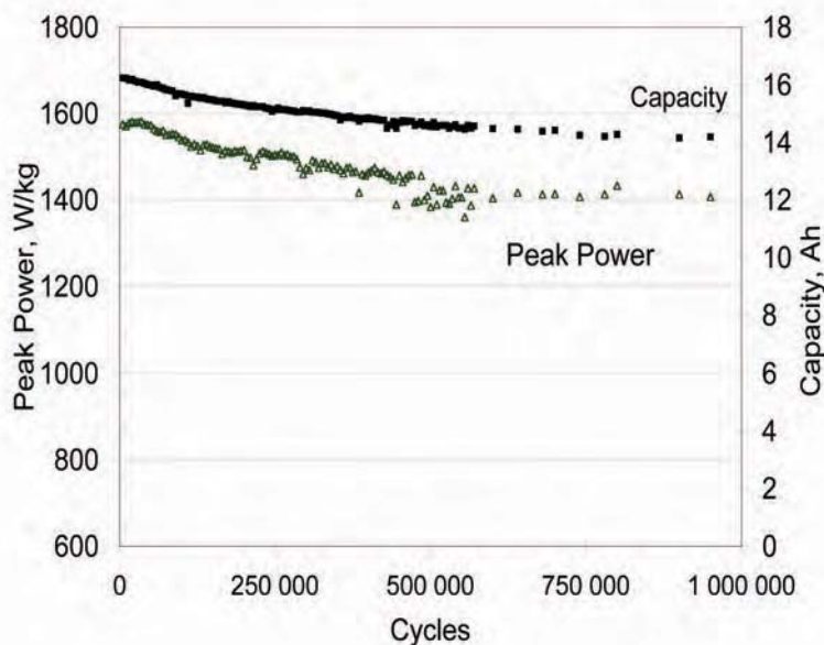
Figure 6: Shallow cycling of high power cell under HEV load profile (periodic 100% DOD diagnostic)
