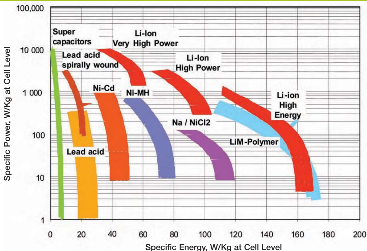
Figure 1: General comparison of main rechargeable systems used in industrial batteries. Pseudo-Ragone diagram W/kg / Wh/kg
