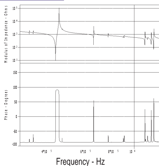
Figure 1: Response of a 455KHz resonator
