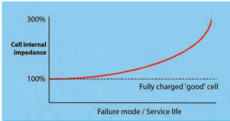
Figure 1 Cell internal impedance is not necessarily a good indicator of impending failure. It is not easy to detect the early stages of failure by this method
