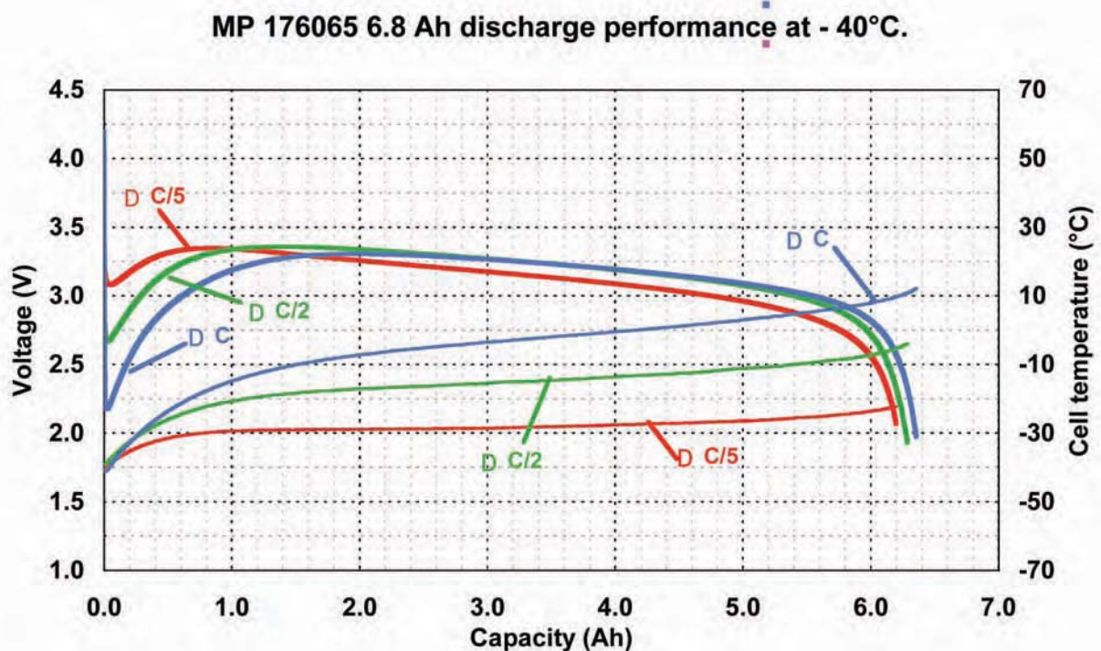
Figure 9: Discharge voltage profile of Saft MP cell at low temperatures
