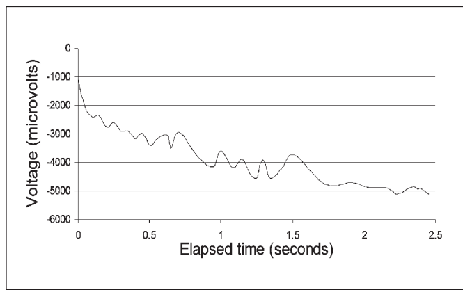
Figure 4b: Underlying trend (splined), with local divergences, for the Figure 4a voltage response to a current-controlled PRBS
