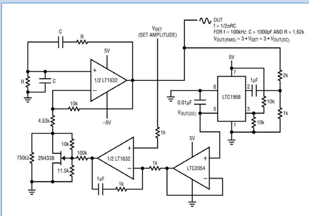
Figure 1: Schematic of the sine wave oscillator, consisting of a low-distortion LT1632-based Wein bridge oscillator core and an LTC1968-controlled amplitude stabilisation loop. The output of the LTC1968 equals the RMS level of the sine wave divided by 3
