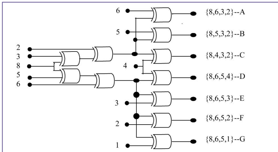
Figure 4: Feedback network
