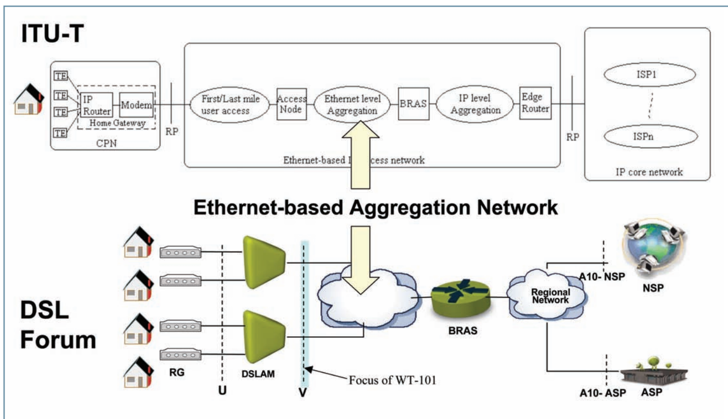
Figure 3: The network architecture for effective delivery of voice, data and video is extremely complex – migrating every element of this structure to IP is far from a trivial task
