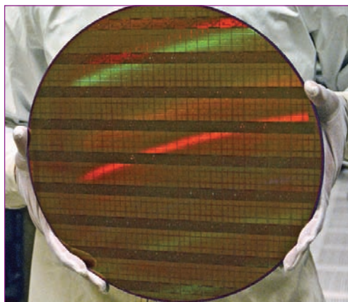
Intel's 300mm wafer with 45nm shuttle test chips
