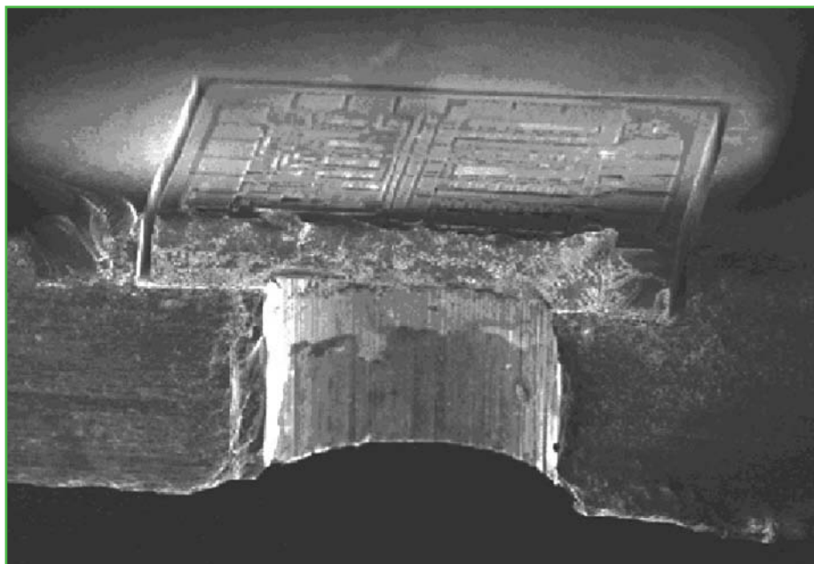
Figure 1: Cross-section cut through a wafer where the chiplet has been inserted into its pit, but the via below has not yet been plated with copper. Note the slight spaces around the edges of the chiplet
