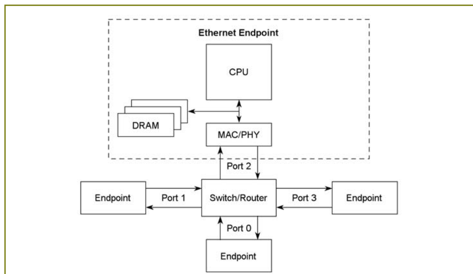
Figure 2: Ethernet was originally designed to connect a large number of powerful computing endpoints in LAN-type configurations. Given its best-effort approach, simple header, addressing for millions of endpoints and single transaction type, the further Ethernet extends down into the system fabric the further its capabilities are stretched to the point where its performance, throughput and reliability begin to appreciably degrade
