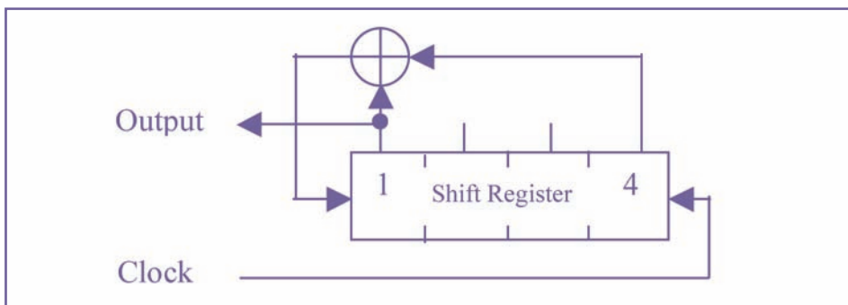
Figure 1: Conventional m -sequence generator
