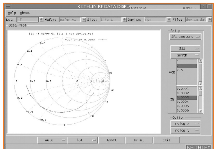
Figure 5: Smith chart
