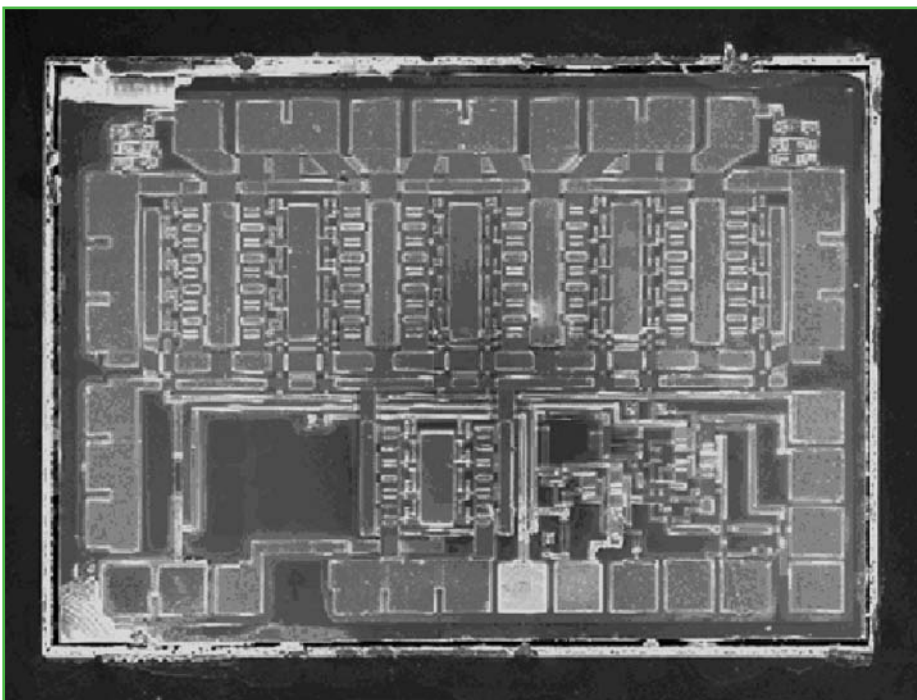
Figure 2: Top view of a chiplet inserted into its pit, before the application of the metallization layer
