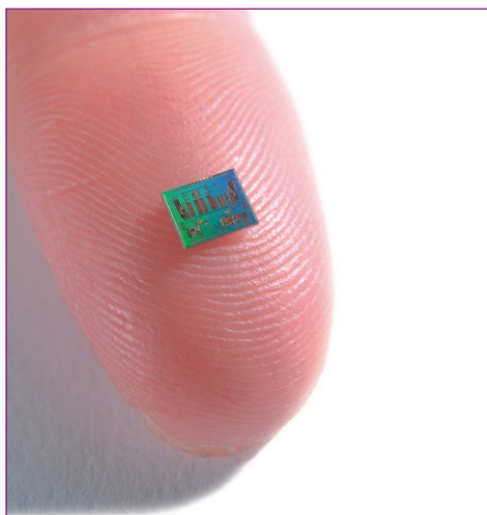
The Scaldio software defined radio transceiver from IMEC
