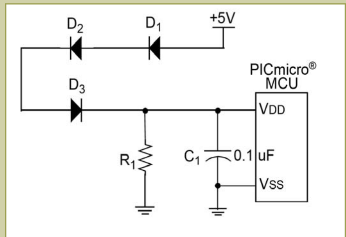
Figure 3: Diode supply
