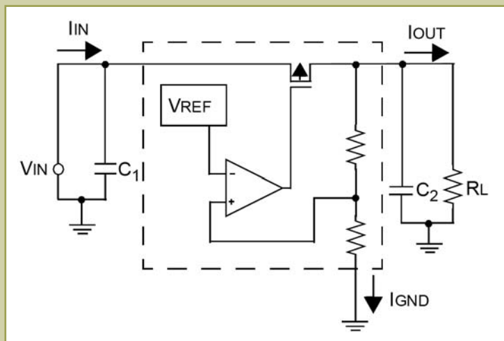
Figure 1: LDO voltage regulator
