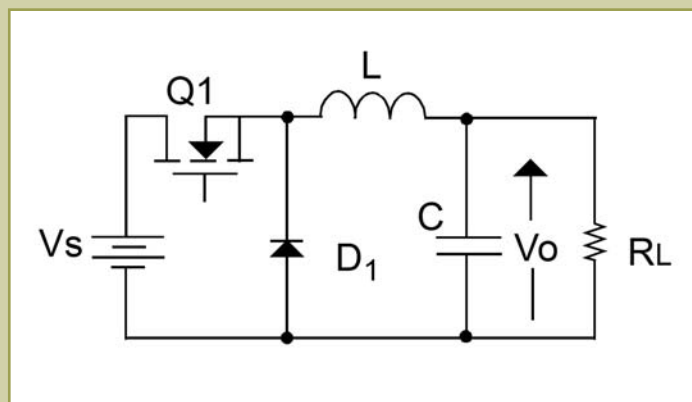
Figure 4: Buck regulator
