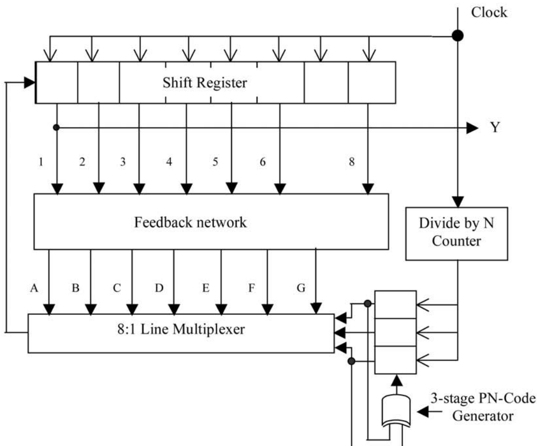
Figure 3: Proposed m-sequence generator
