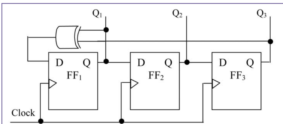
Figure 2: Stage conventional m -sequence generator
