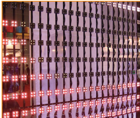
Figure 3 & 4: Multiple LEDs are mounted, with their packaged control electronics, as sub-assemblies on a tape assembly. Multiple tape assemblies are then joined together and a car image on one of these assemblies
