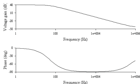
Fig2 Simulated magnitude and phase response of the proposed integrator
