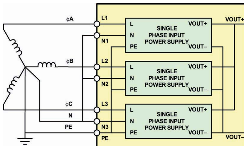
Figure 5: Connecting three single-phase input ac-dc power supplies for operation from three-phase wye ac power
