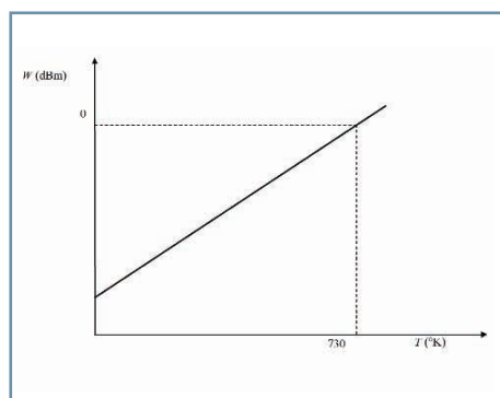
Figure 1: Received noise power ( W ) from the hot object in function of its temperature T
