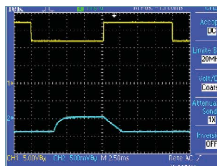
Figure 8: LNB preamplifier V_{gs} and V_{ds} .
