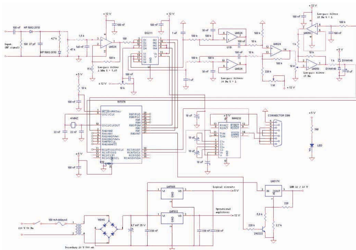
Figure 4: Electrical diagram
