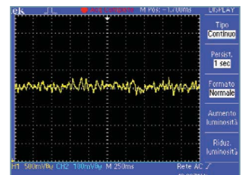
Figure 9: Input PIC16F876A AD converter (without signal).
