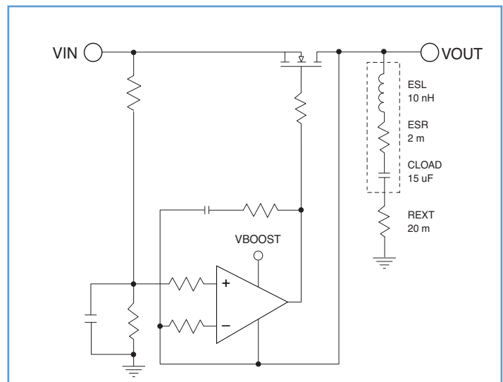
Figure 4 Typical active output filter (QPO series from Picor)
