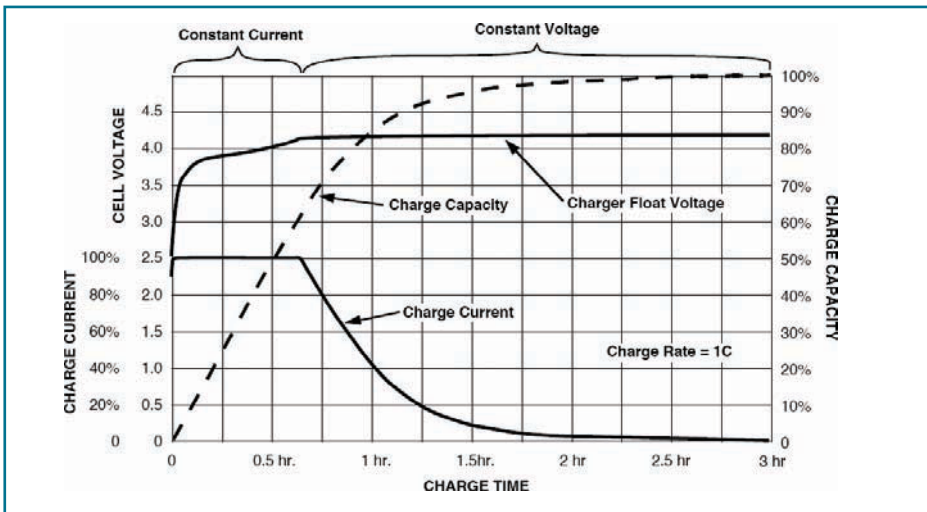
Figure 2: Typical charge profile showing battery current, voltage and capacity
