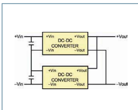
Figure 4: Series input, parallel output technique for reducing converter input voltage
