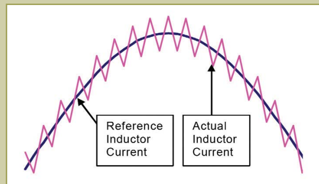
Figure 2: Desired and actual inductor currents
