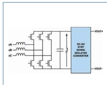
Figure 3: Conceptual diagram of a three-phase input ac-dc power supply
