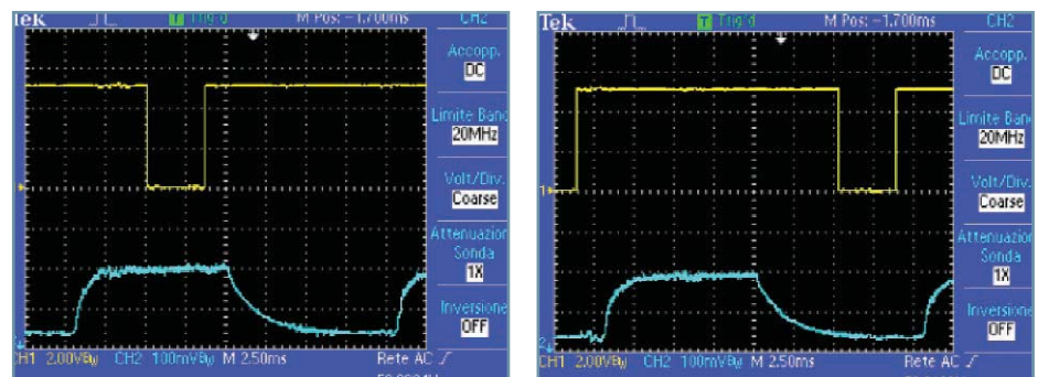
Figure 7: Switch closing - horizontal polarisation (left, up trace), switch closing - vertical polarisation (right, up trace), detector output (down trace)
