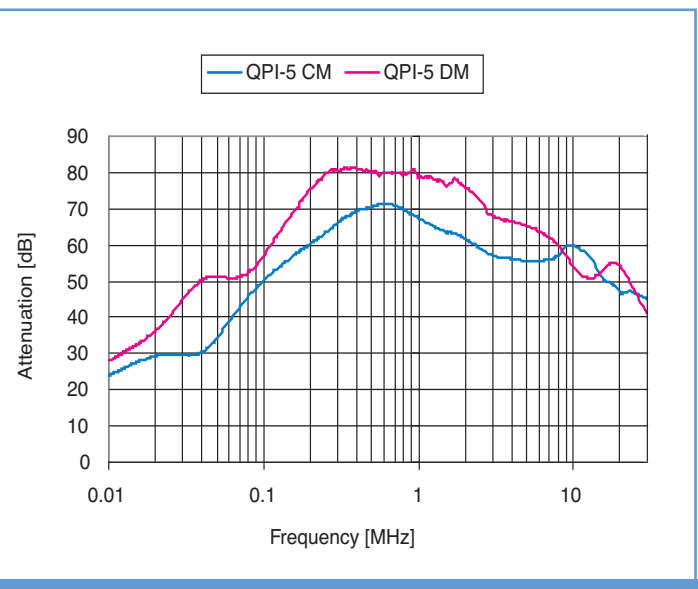
Figure 2: Attenuation curves for common and differential mode performance for the active solutions
