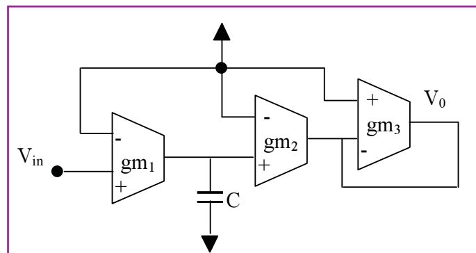
Figure 3: Proposed integrator
