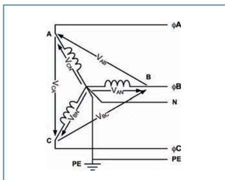
Figure 2: Three-phase wye connection with neutral and protective earth wires
