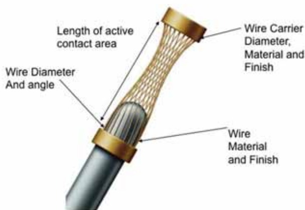
Figure 2: Design parameters of the Hyperboloid socket contact
