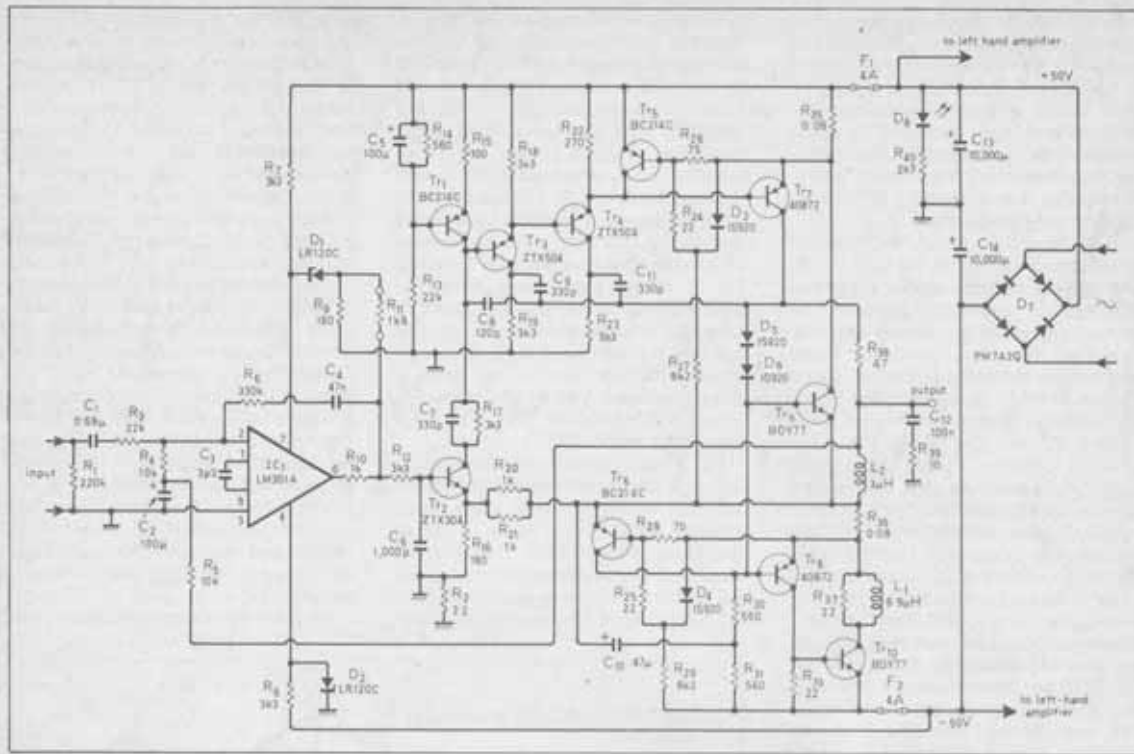
Fig. 4. Full circuit diagram. Resistor R_2 is a protective connection provided to ensure earth continuity in the event that Tr_2 and its associated component panel are disconnected from the common earth chassis.
