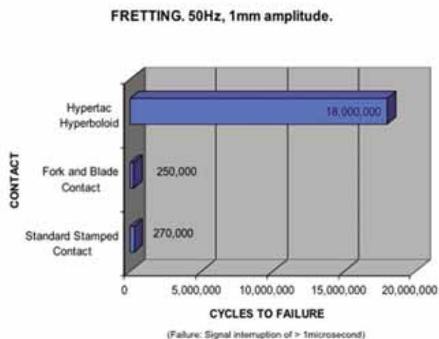
Figure 3: Fretting corrosion characteristic of Hyperboloid contacts
