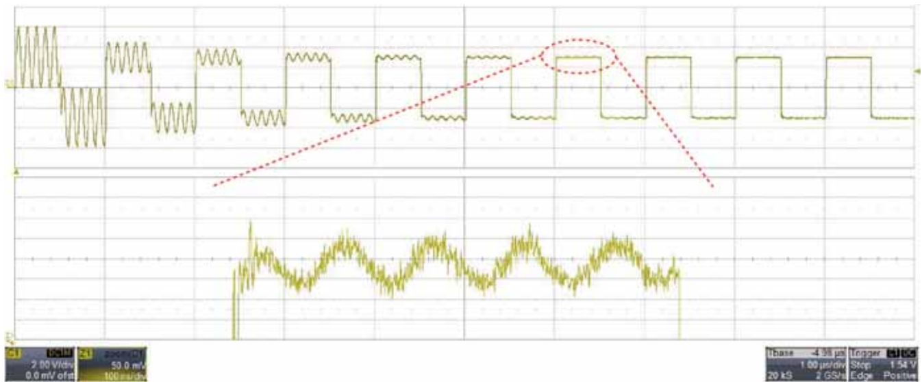
Figure 4: Because HD4096 technology achieves true 12-bit resolution through hardware improvements and not through averaging or filtering, the user no longer needs to average samples by combining multiple acquisitions into a single trace. Compare this HDO screen image with Figure 2, which illustrates the result of multiple-acquisition averaging
